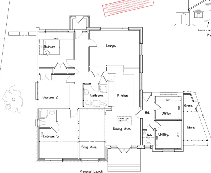
Proposed Layout.
